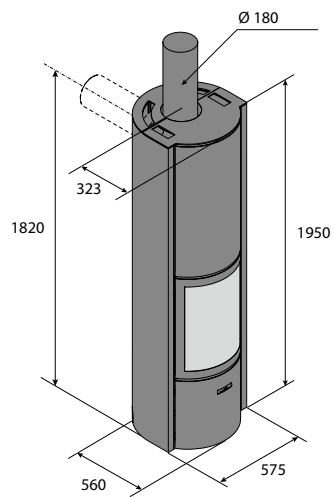
Stûv 30-H
